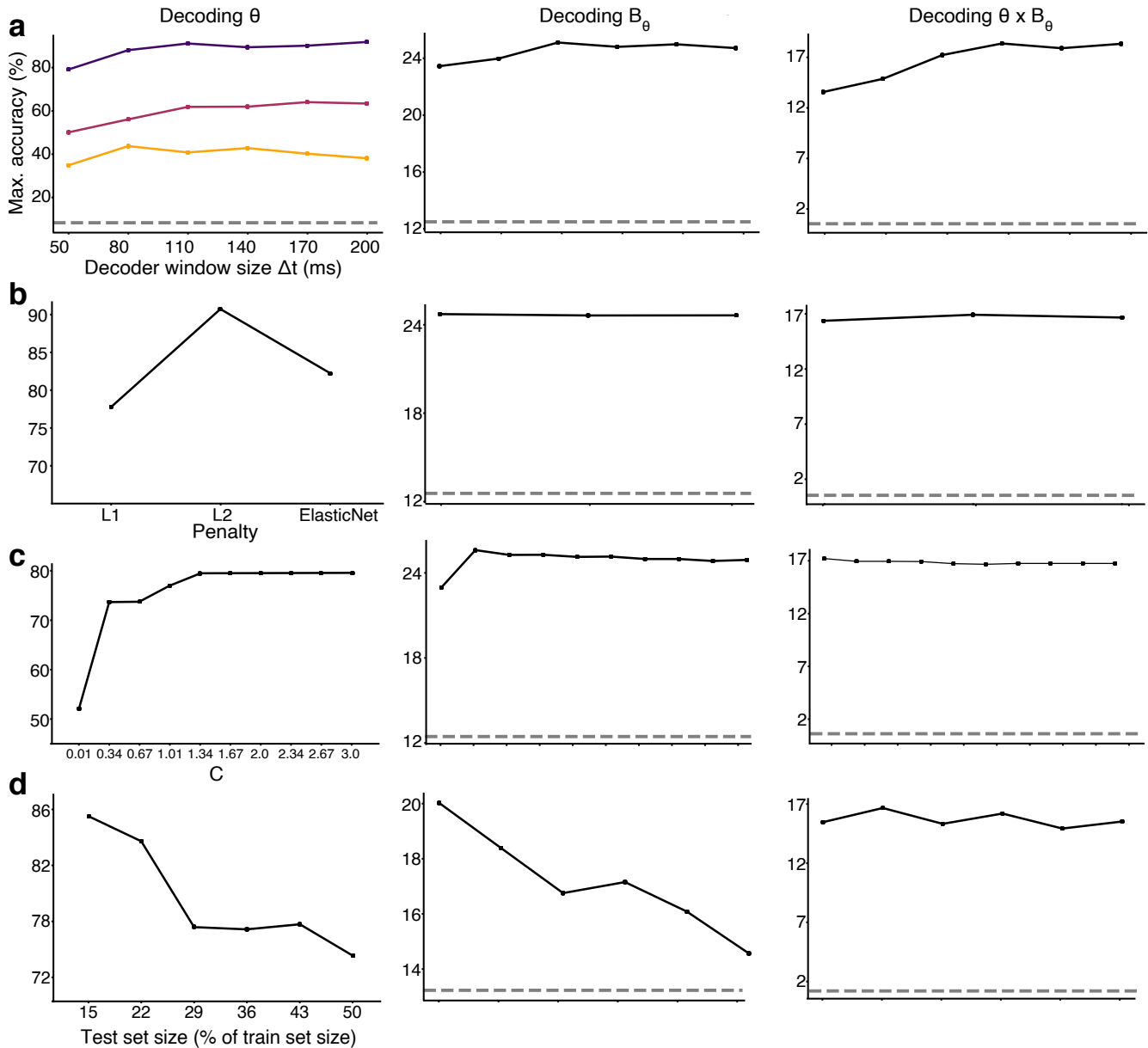
Supplementary Figure 6. Parameters evaluation of the decoders. (a) Optimization of the length of the time window \Delta T , which controls the length of the integration time of the decoder (see Methods), for orientation decoders (left column), variance decoders (middle column) and orientation x variance decoders (right column). (b) Optimization of the penalization norm applied to the decoder, which controls the metric by which the classification error is minimized. l_1 and l_2 are defined as \sum_i |x_i| and \sqrt{\sum_i |x_i|^2} , where x is a set of features fed to the classifier. The penalty norm ElasticNet linearly combines these two norms, here with equal weighting applied to both norms. (c) Optimization of the parameter C controls the regularization strength, which measure the magnitude of the penalty applied to large parameters, in order to prevent overfitting on reduced sets of data. (d) Optimization of the percentage of data kept out of the training set to evaluate the decoder's accuracy.
